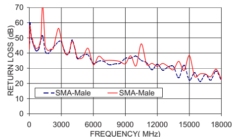
141-4SM+ RETURN LOSS
