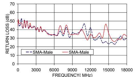
141-9SM+ RETURN LOSS
