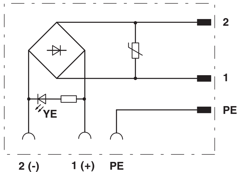
Circuit diagram
