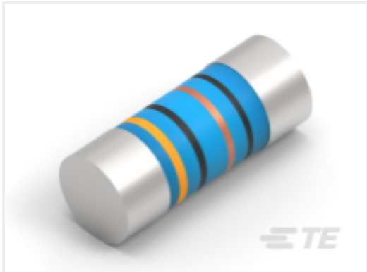
TE Part #6-2176316-9 MELF SMA_A 39K 1% 50PPM 0207 1W
