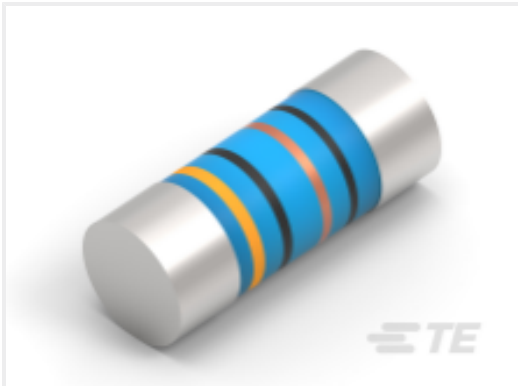
TE Part #5-2176316-2 MELF SMA_A 1K5 1% 50PPM 0207 1W
