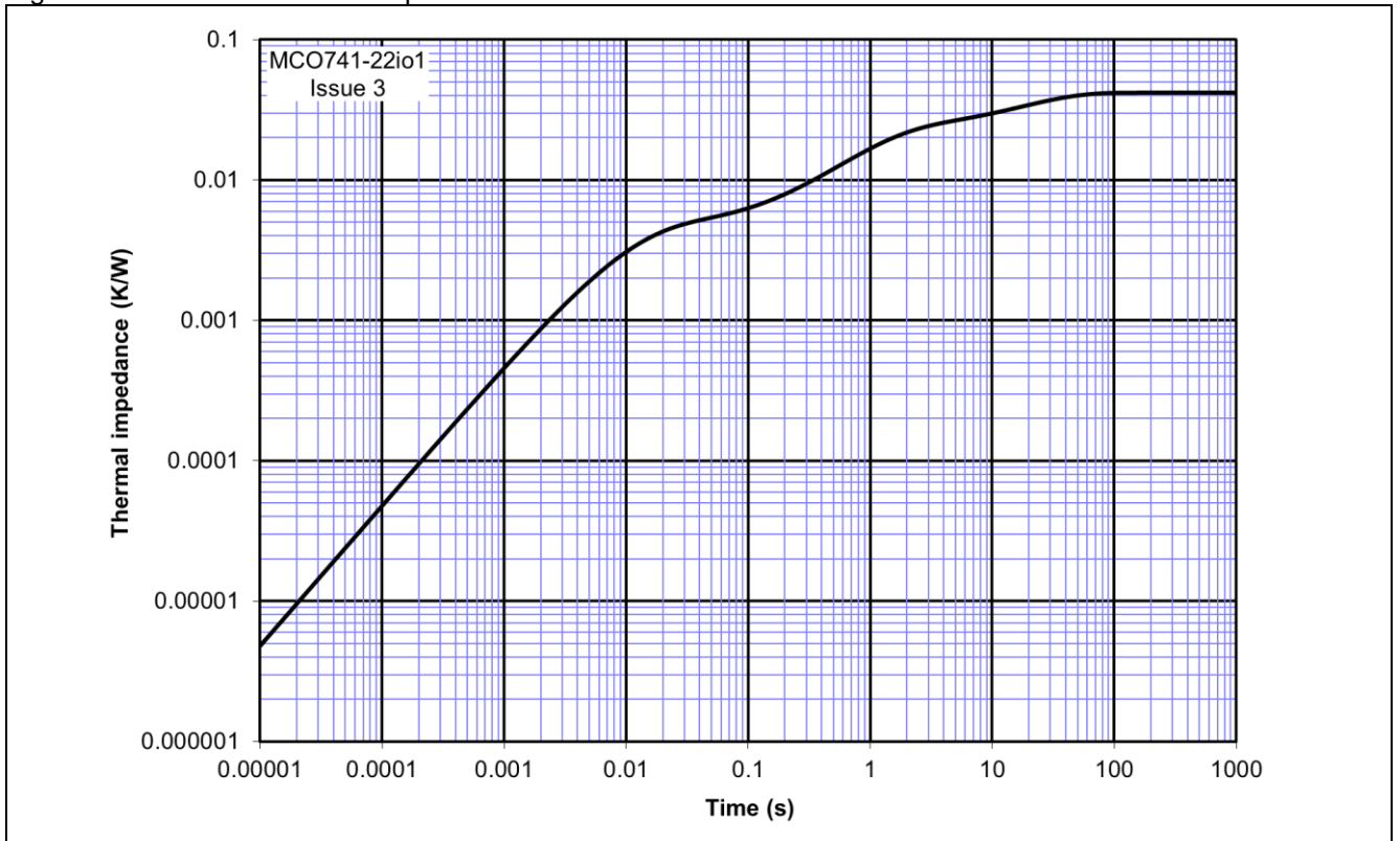
Figure 9 – Transient Thermal Impedance
