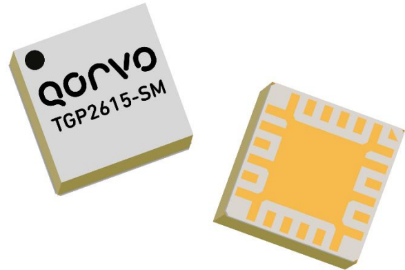
Air Cavity Ceramic QFN 4x4 mm 24L
